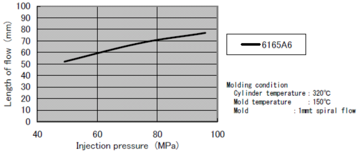
(Figure 3-1) Flowability(1mmt)
